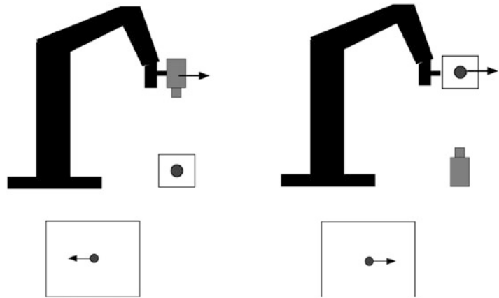
Visual Servoing, Fig. 2 If the goal is to move the camera from frame R_c to the desired frame R_{c^*} , two main approaches are possible: IBVS on the left, where the
