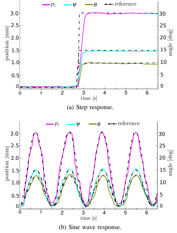
Fig. 3. 3-DoF cutaneous device. Performance of the decoupled position control scheme shown in Fig. 2b.
