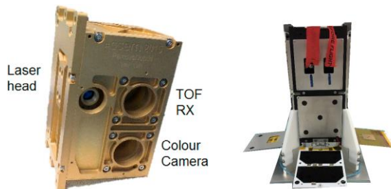
Figure 4. Left: Vision Based Navigation payload, Right: DS-2 target in deployed state
