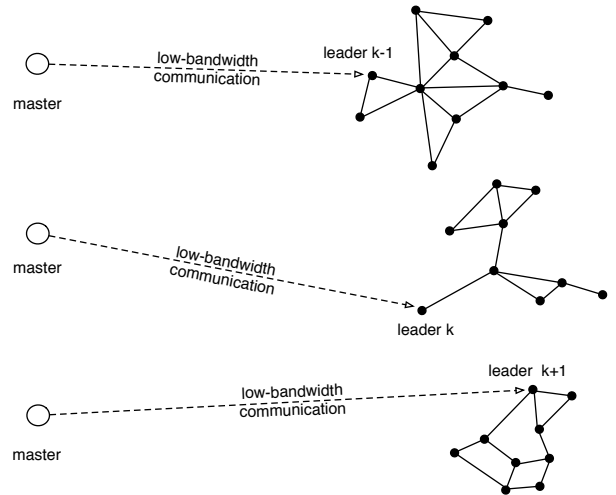
Fig. 1: Abstraction of the application scenario, in which a master agent (e.g., a base station) can only communicate with one an agent at the time (called leader) with a low bandwidth. The leader can be changed every time a new high-level command from the master is sent to the group.
