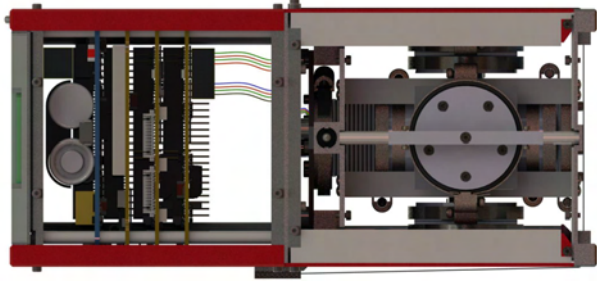
(a) Undeployed Structure
