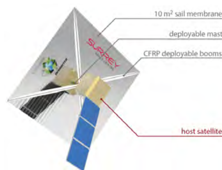
Fig. 31: Dragsail Concept.
