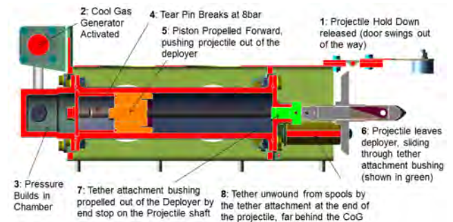
Fig. 22: Harpoon Firing Process.
