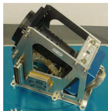
Fig. 33: Supervision Camera. With housing.
