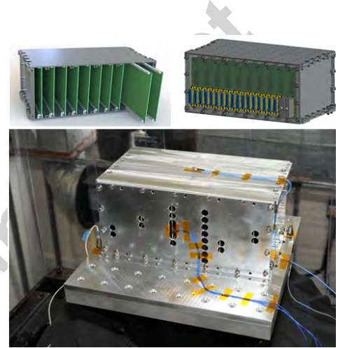
Fig. 9: Platform: Card Frame Assembly.
