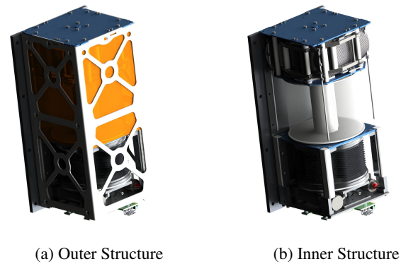
Fig. 32: Dragsail Payload
