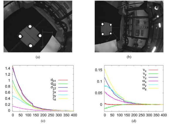
Fig. 15. Rotation and translation displacement. (a) Desired image, (b) initial image, (c) errors, and (d) computed camera velocities (in meters per second and radians per second).
