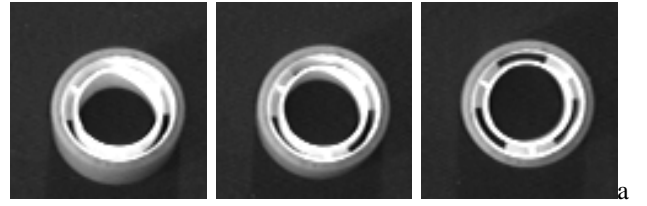
Fig. 3. [Real experiment] Positioning wrt. a sphere (a) first image (b-c) luminance increases (d) the camera is now between the sphere and the light (that is the actual expected position but that in practise create a “light occlusion”)
